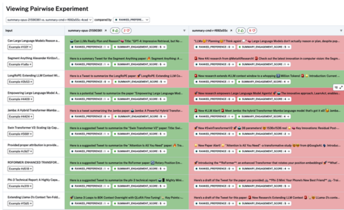
Figure 10-13. Pairwise experiment UI evaluation trace
