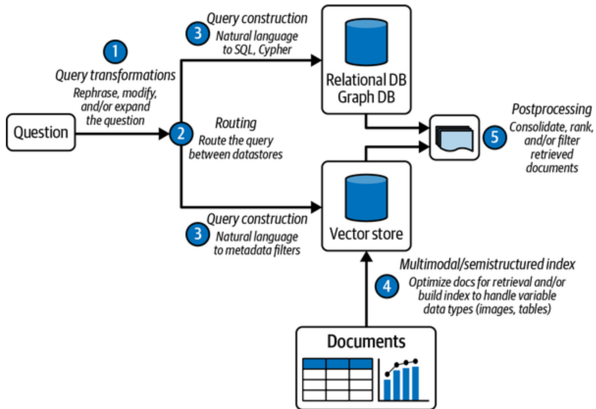
Figure 3-4. Effective strategies to optimize the accuracy of your RAG system
