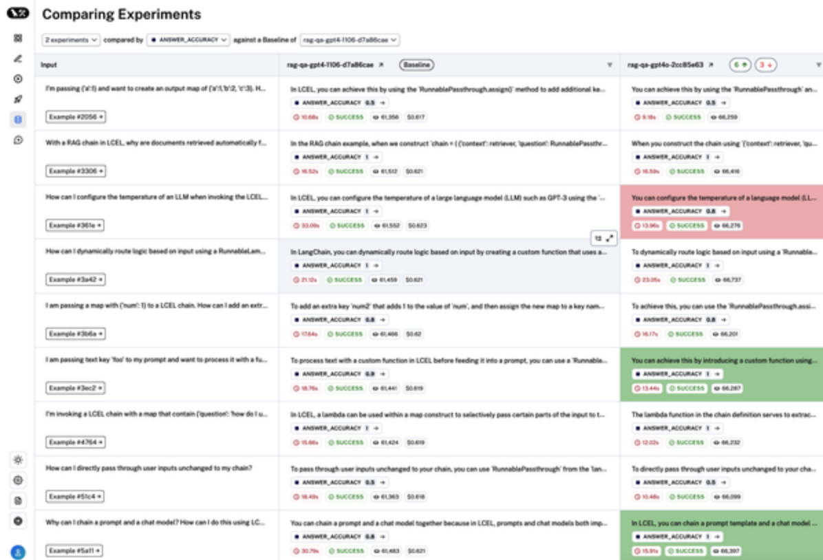
Figure 10-14. LangSmith's experiments comparison view
