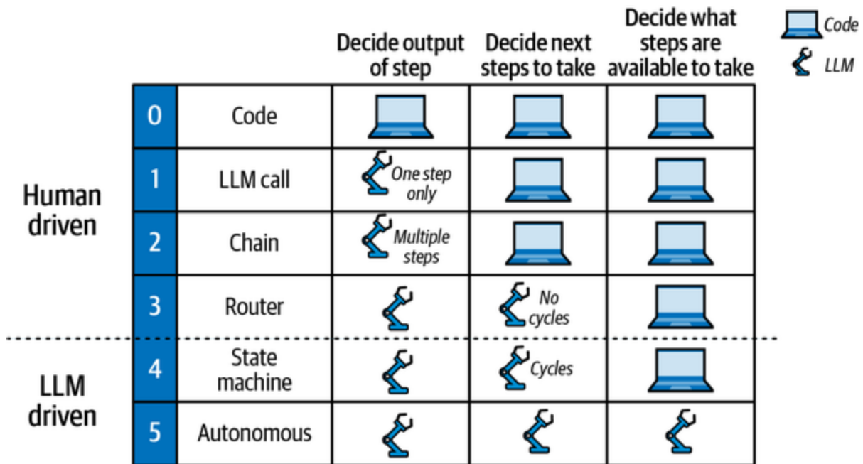
Figure 5-1. Cognitive architectures for LLM applications
