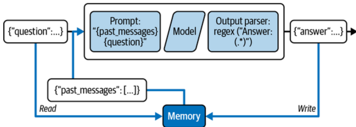
Figure 4-2. A simple memory system utilizing chat history in prompts to generate model answers
